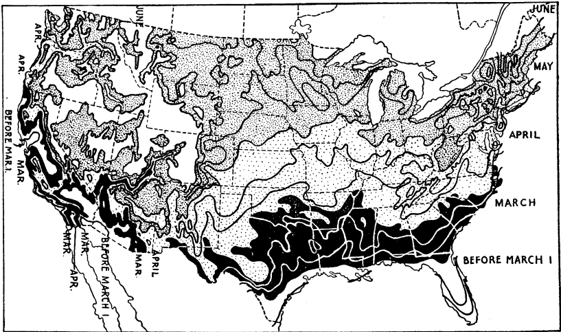
FIGURE 9.—Outline map of the United States showing the date of the average occurrence of the last spring frost
